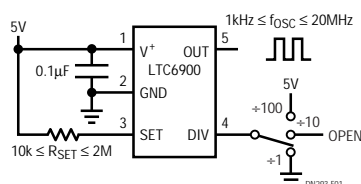
Figure 1. Basic Connection Diagram
