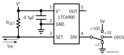
Figure 3. Concept for Programming via Current Steering
