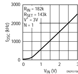
Figure 6. Output Frequency vs Input Voltage
