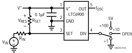
Figure 4. Implementation of the Concept Shown in Figure 3
